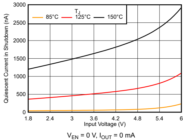
Figure 6-13. Shutdown Current vs V_{IN}
