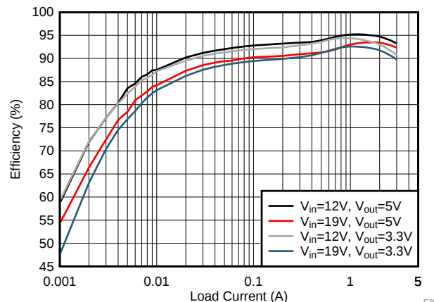
TPS56339 Efficiency
