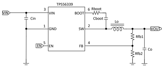
Simplified Schematic
