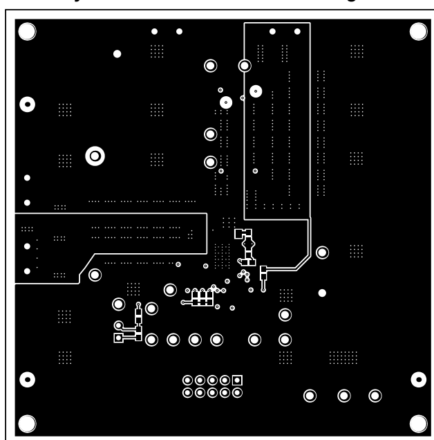
Figure 67. EVM Bottom Layer
