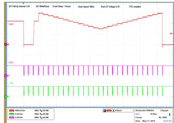
Figure 20. 29 Sequenced Events – I2C Write
