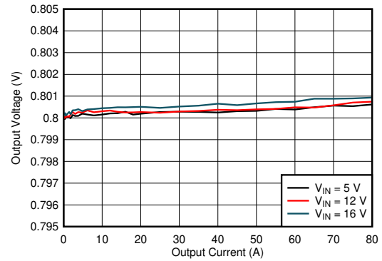
Figure 8-13. Load Regulation
