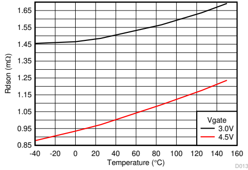
Figure 6-13. Low-Side MOSFET On-Resistance (R DS(on) ) vs Junction Temperature
