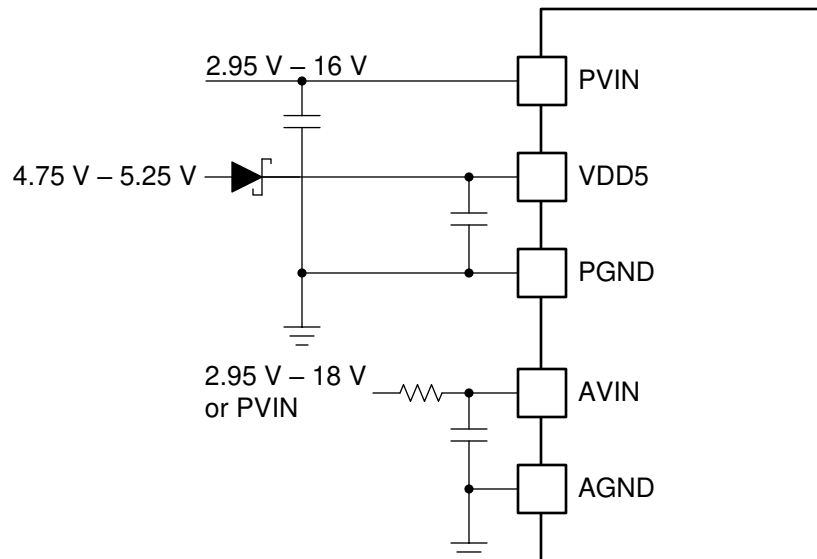
Figure 7-4. TPS546D24A Separate PVIN, AVIN, and VDD5 Connections
