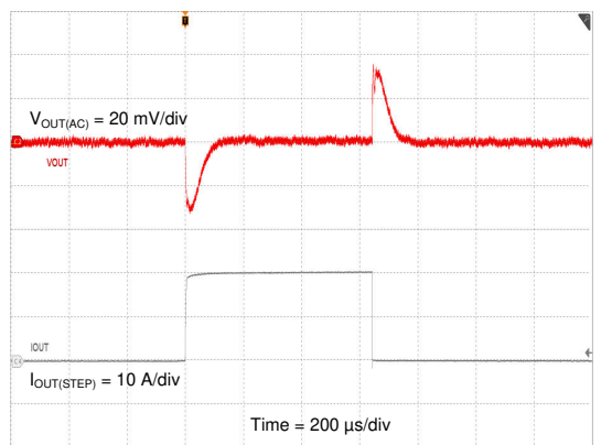
Figure 8-14. Load Regulation
