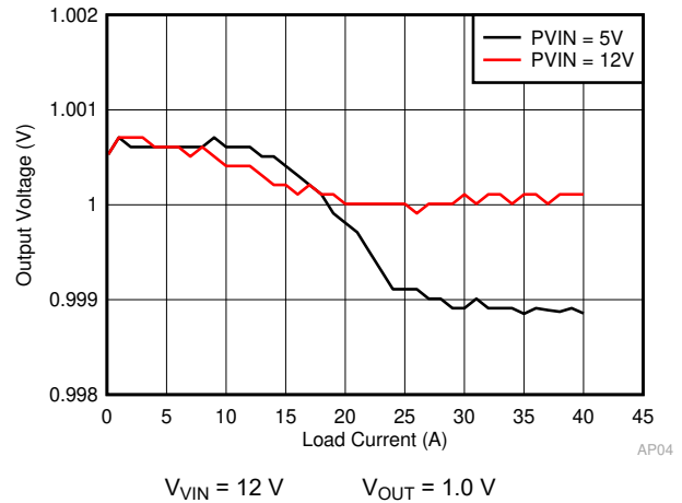
Figure 8-3. Load Regulation
