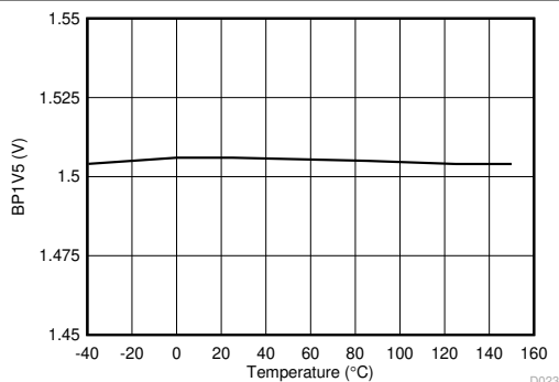
Figure 6-19. BP1V5 Voltage vs Junction Temperature
