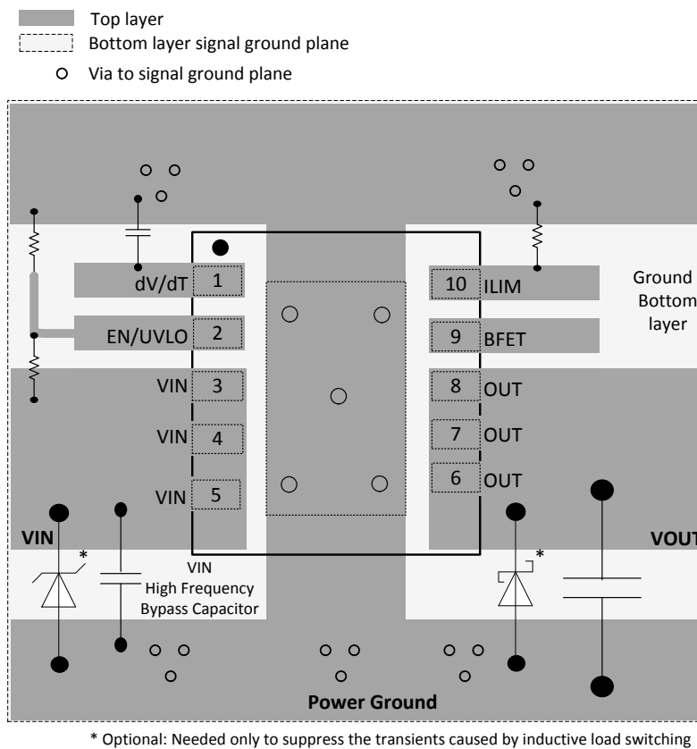
Figure 43. Layout Example
