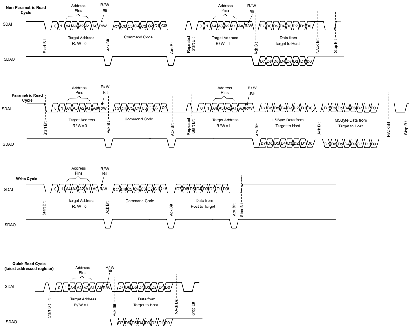
Figure 9-4. I²C interface Read and Write Protocol – Configuration A
