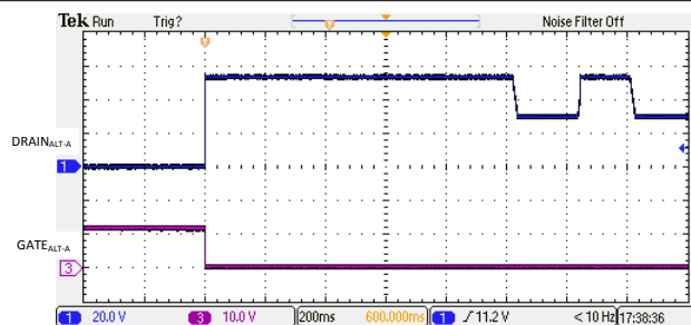
Figure 10-4. Backoff Due to PCut Fault
