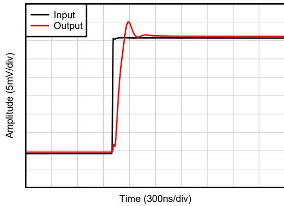
C_L = 20\text{ pF} , G = 1 , 20-mV step response C010
