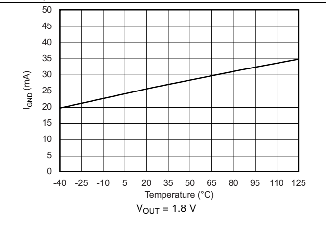
Figure 8. Ground Pin Current vs Temperature
