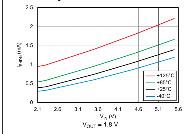
Figure 9. Shutdown Current vs Input Voltage
