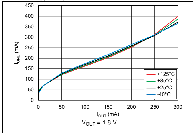
Figure 7. Ground Pin Current vs Load
