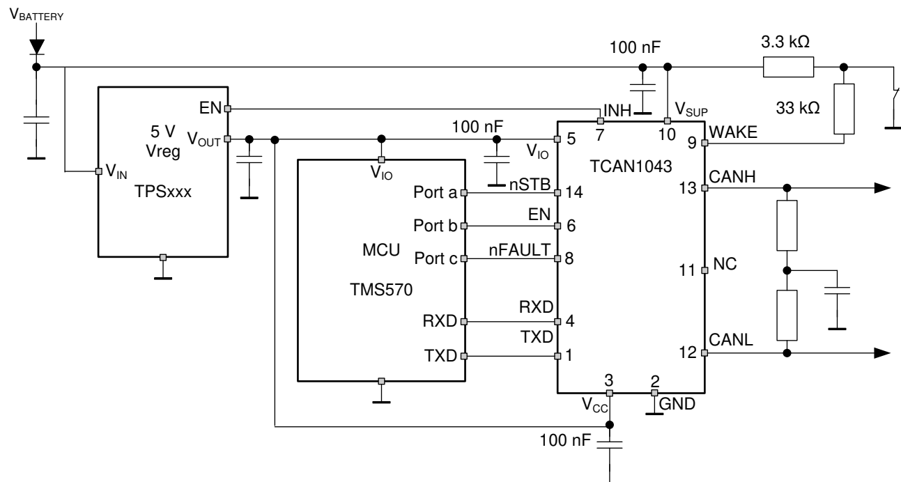
Figure 10-1. Typical CAN Bus Application Using TCAN1043xx-Q1 with 5 V \mu C
