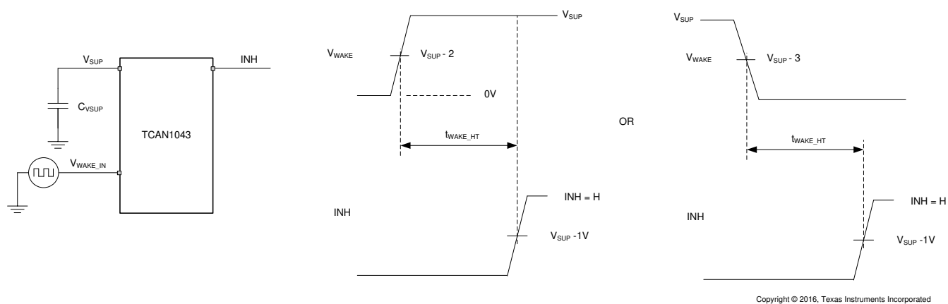
Figure 8-12. t_{Wake\_HT} While Monitoring INH Output
