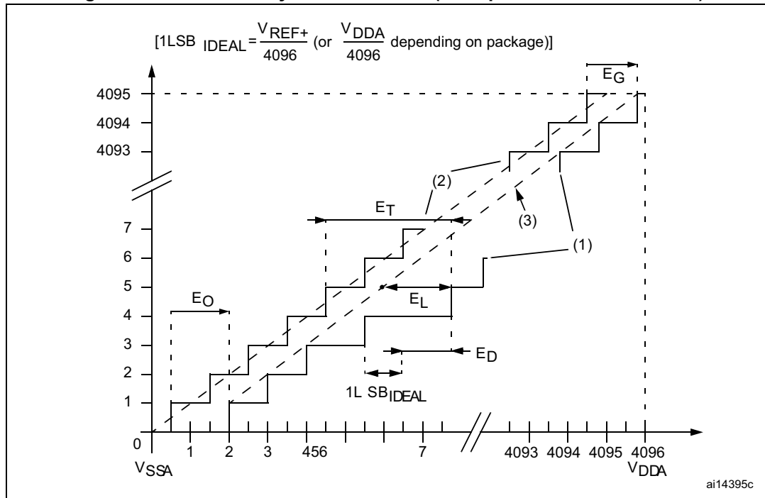
Figure 88. ADC accuracy characteristics (example for 12-bit resolution)
