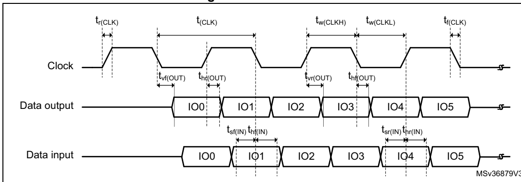
Figure 113. DDR mode
