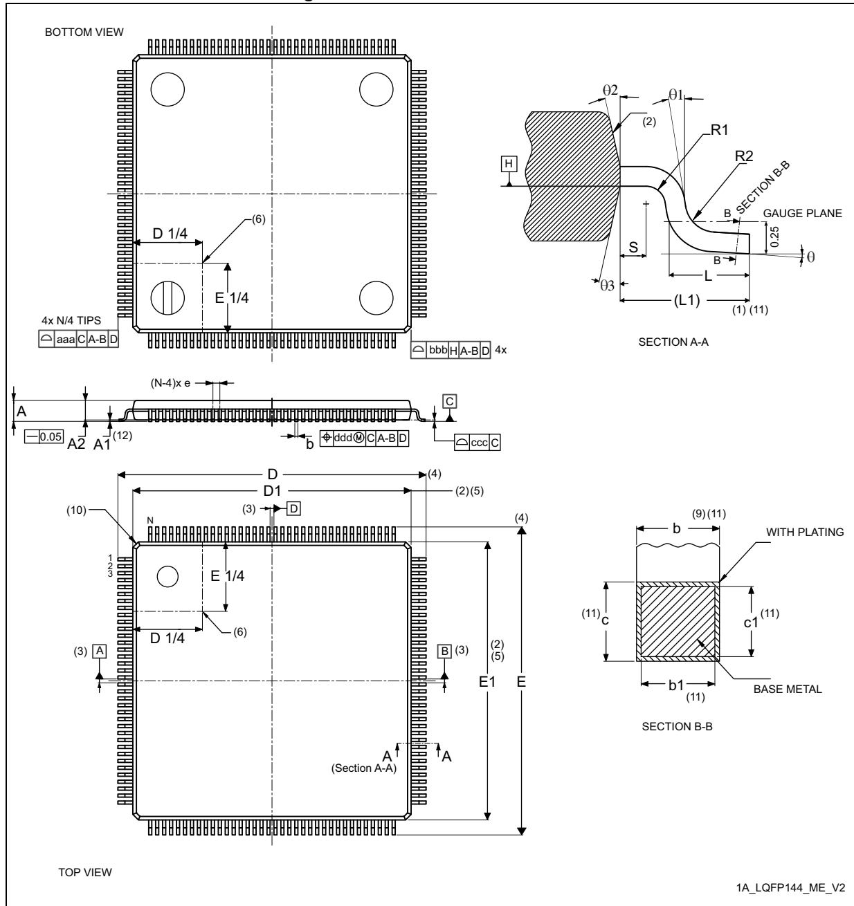
Figure 126. LQFP144 - Outline (15)
