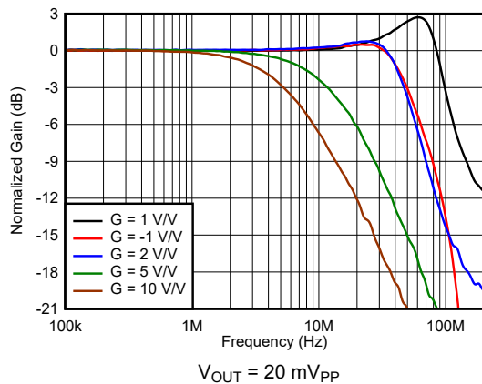
Figure 7-31. Small-Signal Frequency Response vs Gain
