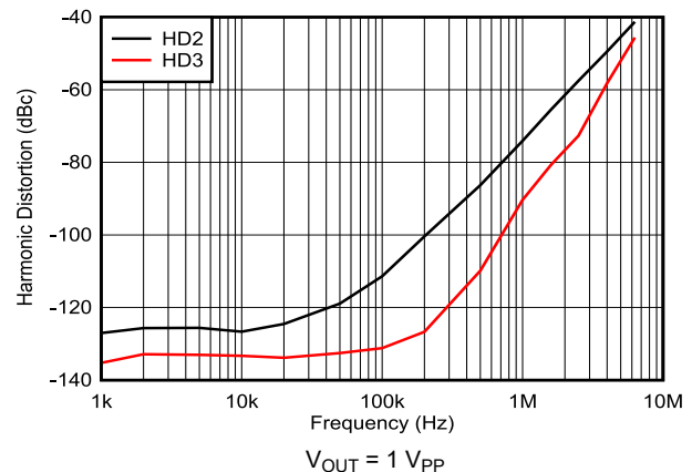
Figure 7-32. Harmonic Distortion vs Frequency
