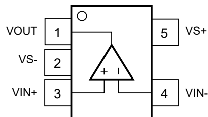
Figure 6-2. DBV Package, 5-Pin SOT-23 (Top View)
