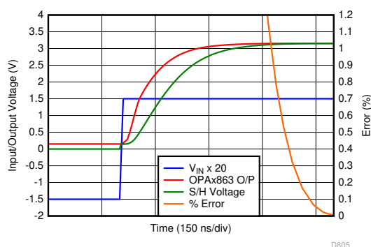
Figure 9-2. 0.1% Settling Performance
