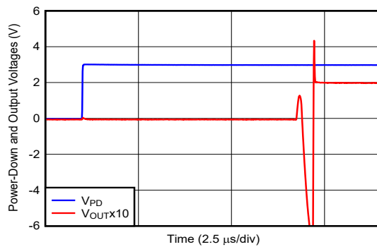
Figure 7-39. Turn-On Time to DC Input
