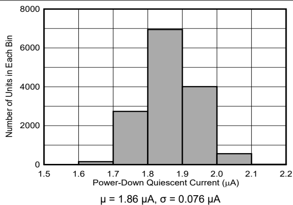
Figure 7-29. Power-Down Quiescent Current Distribution
