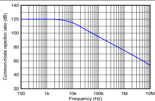
Figure 7-47. Common-Mode Rejection Ratio vs Frequency
