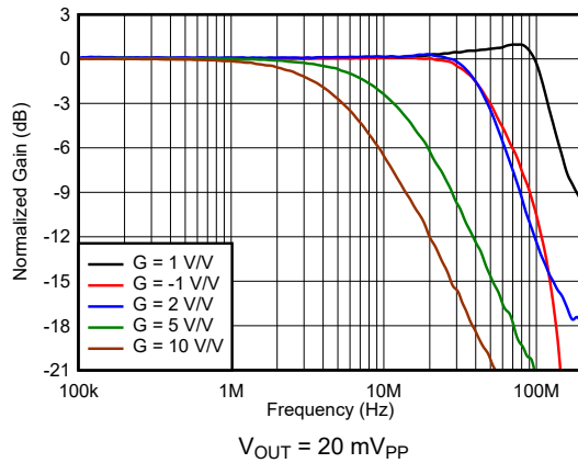
Figure 7-1. Small-Signal Frequency Response vs Gain
