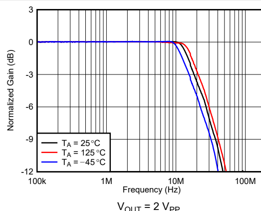
Figure 7-8. Frequency Response vs Ambient Temperature
