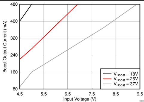
Figure 1. Maximum Boost Current
