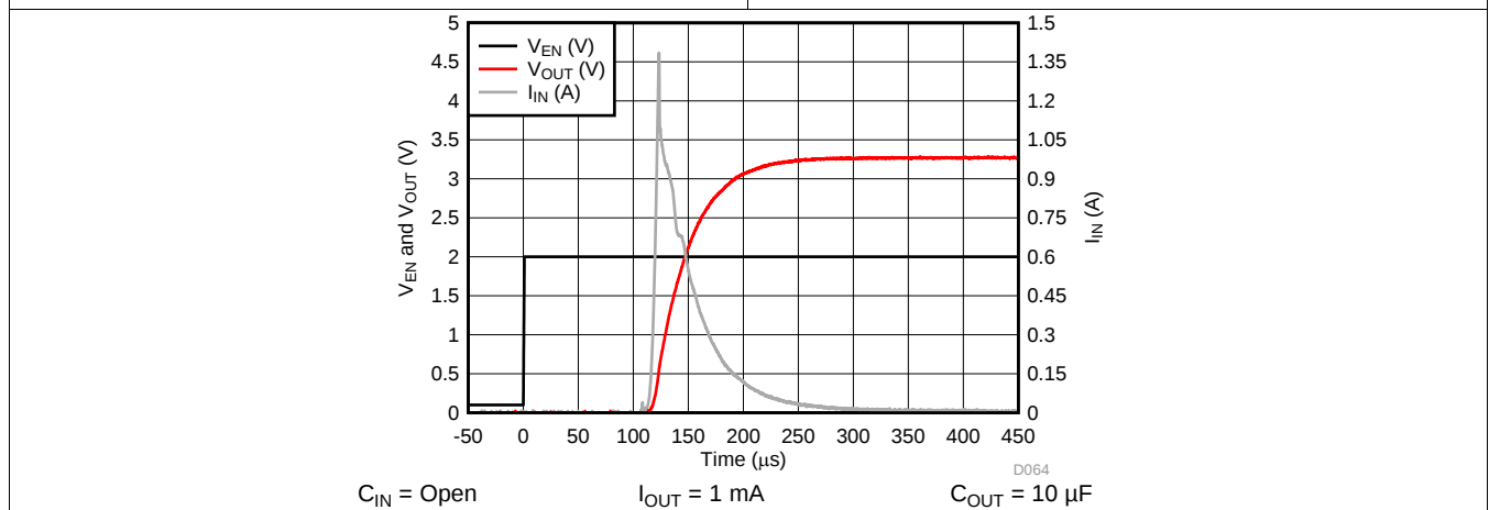
Figure 51. LP5912-3.3 In-Rush Current
