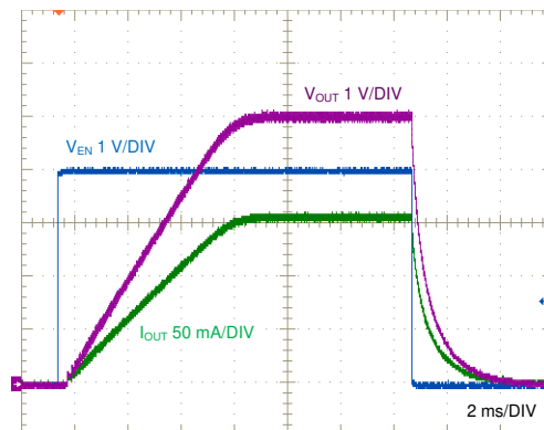
V_{IN} = 24 V 30- \Omega Load
