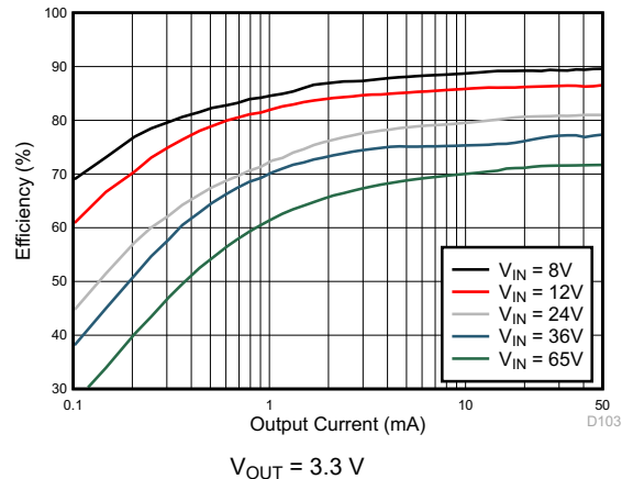
Figure 8-15. Efficiency
