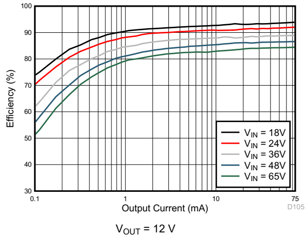
Figure 8-22. Efficiency
