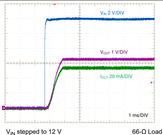
Figure 8-17. Start-Up, Full Load
