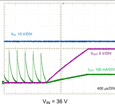
Figure 8-35. Short Circuit Recovery
