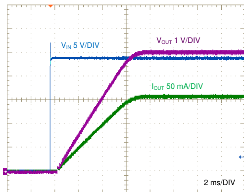
V_{IN} stepped to 24 V 30- \Omega Load
