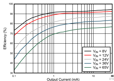
Typical Efficiency, V_{OUT} = 5\text{ V}
