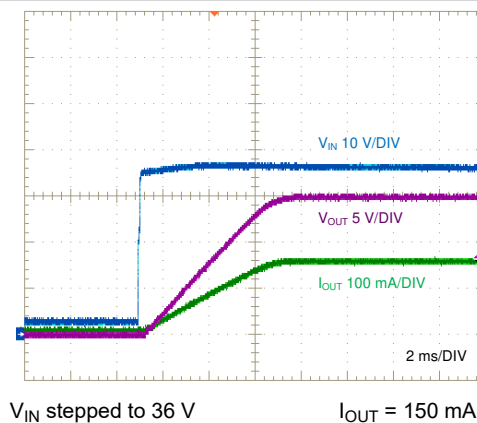
Figure 8-31. Start-Up, Full Load
