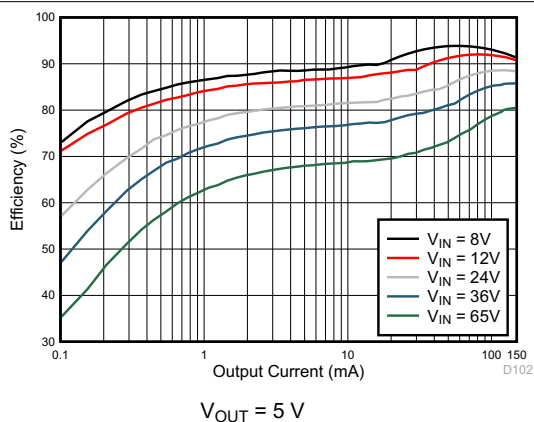
Figure 8-2. Efficiency
