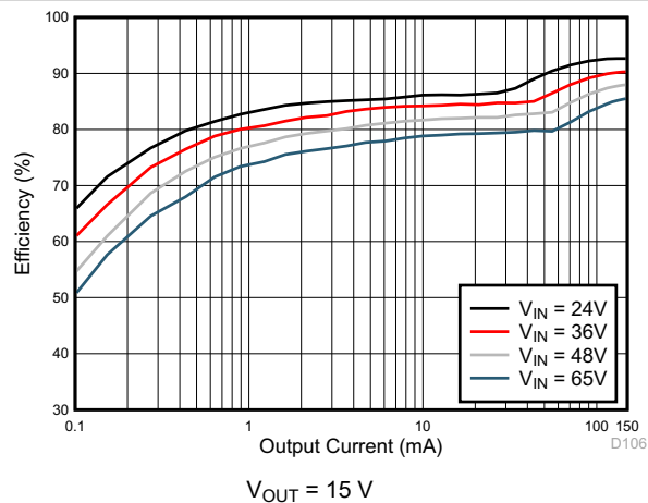
Figure 8-30. Efficiency
