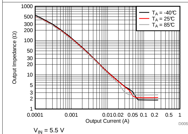
Figure 5. Output Impedance vs Output Current
