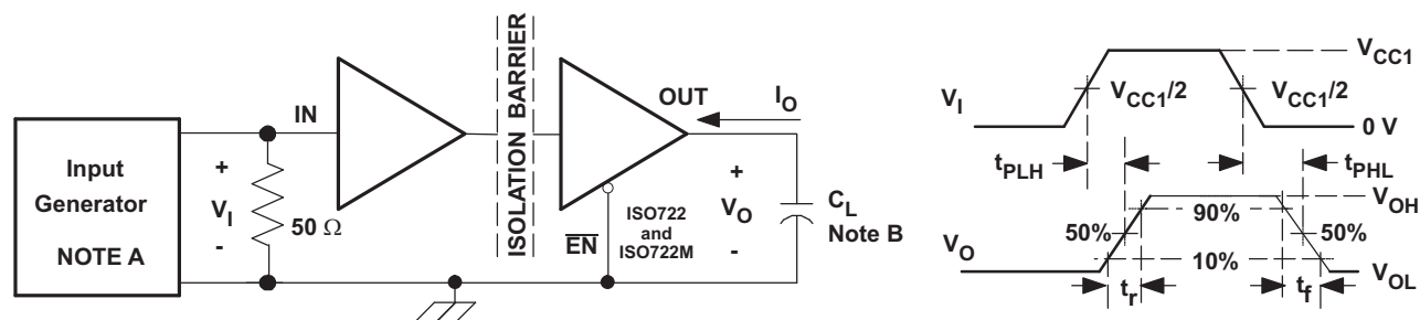
Figure 10. Switching Characteristic Test Circuit and Voltage Waveforms
