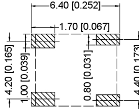
Recommended P.C.B Layout General Tolerances:0.05
