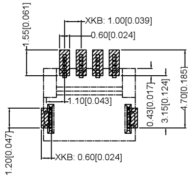
Recommended P.C.B. Layout Total tolerance:±0.05mm
