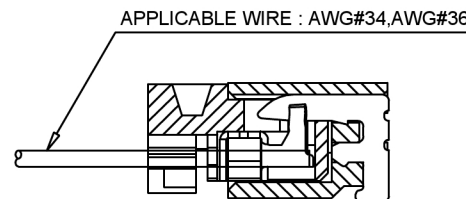
MATED CONDITION
