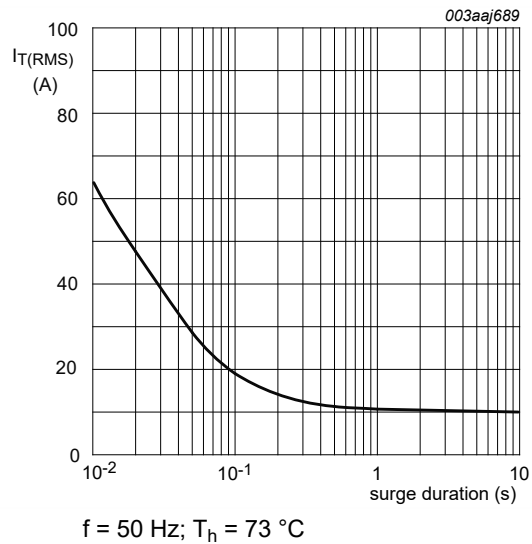
Fig. 2. RMS on-state current as a function of surge duration; maximum values f = 50 Hz; T h = 73 °C
