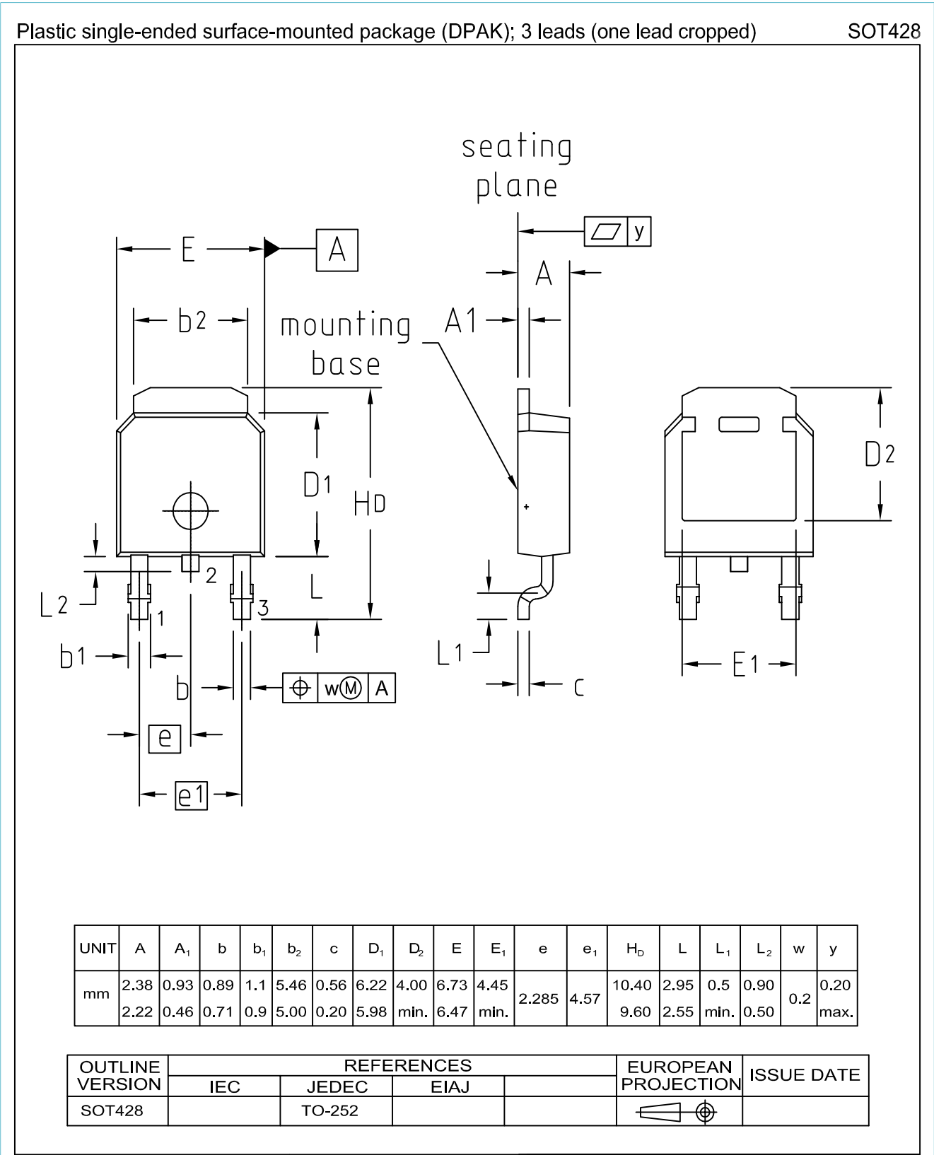
Fig. 16. Package outline DPAK (SOT428)
