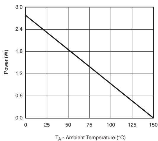
Power, Junction-to-Ambient
