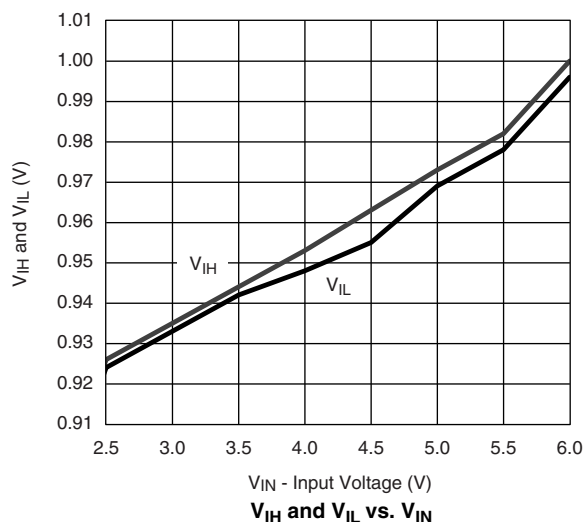
V_{IH} and V_{IL} vs. V_{IN}
