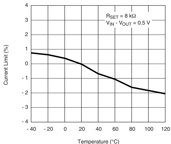
Current Limit vs. Temperature
