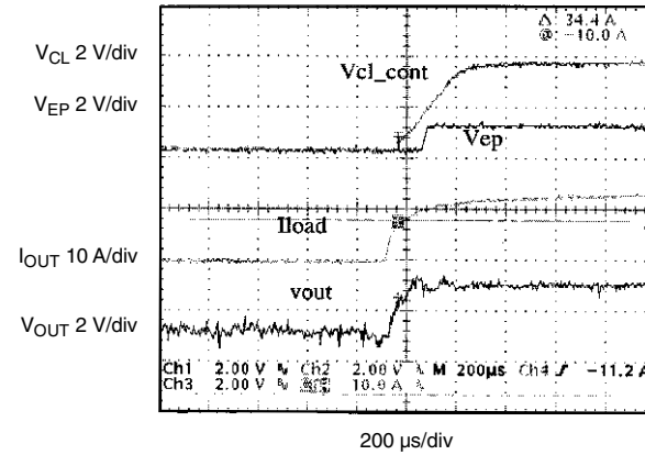
Figure 10. Overload Recovery
