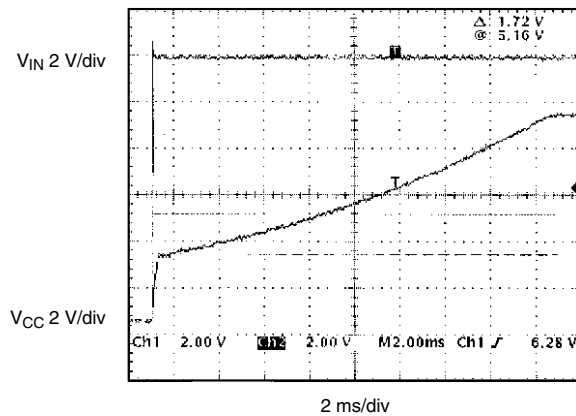
Figure 9. V_{CC} Ramp-Up
