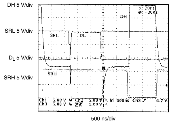
Figure 12. Drive Waveforms
