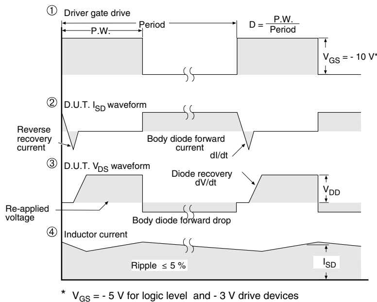
Fig. 14 - For P-Channel
