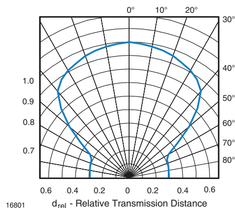
Fig. 3 - Horizontal Directivity
