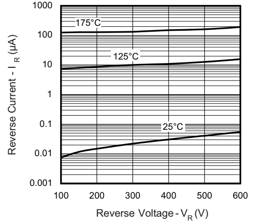
Fig. 1 - Typical Values of Reverse Current vs. Reverse Voltage
