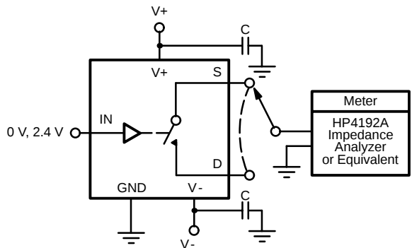
FIGURE 6. Source/Drain Capacitances
