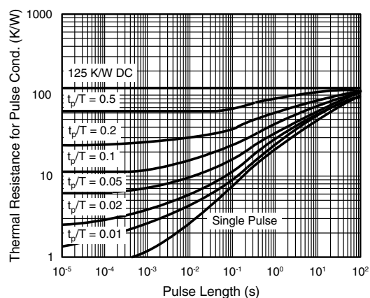
Fig. 8 - Thermal Response
