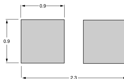
Dimensions of the solder lands.
