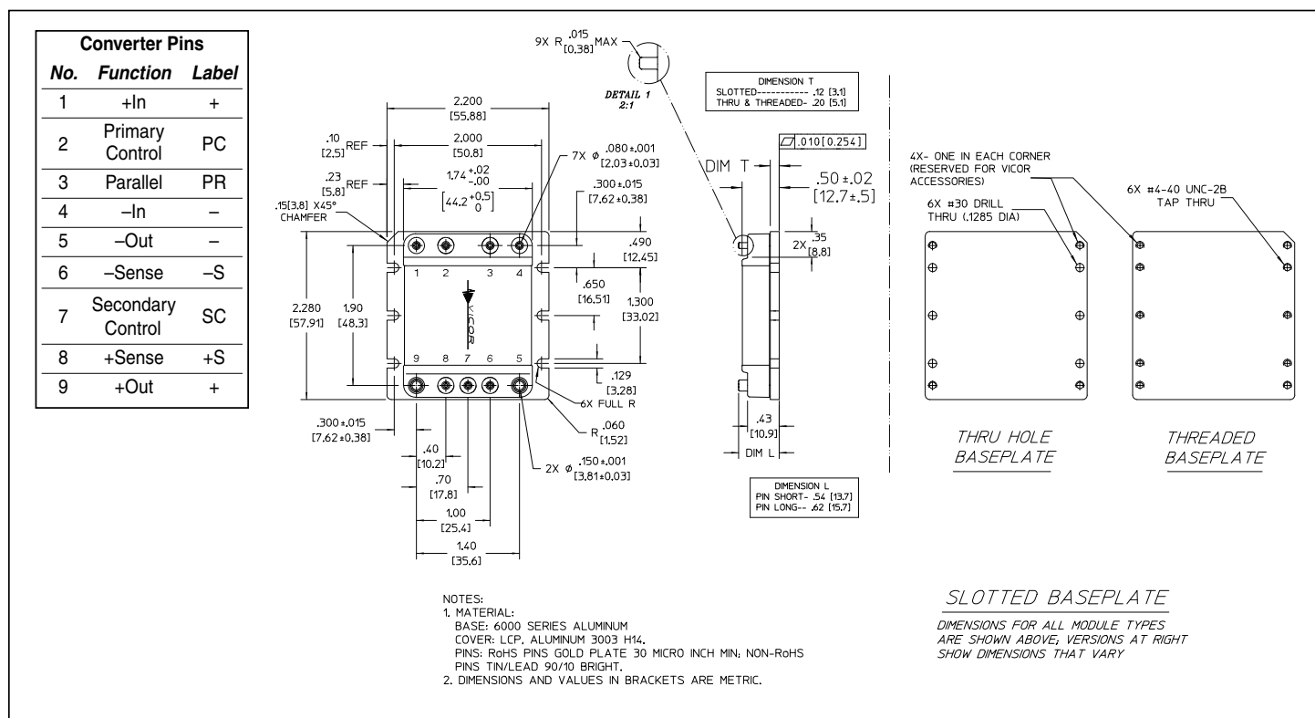
Figure 12 — Module outline
