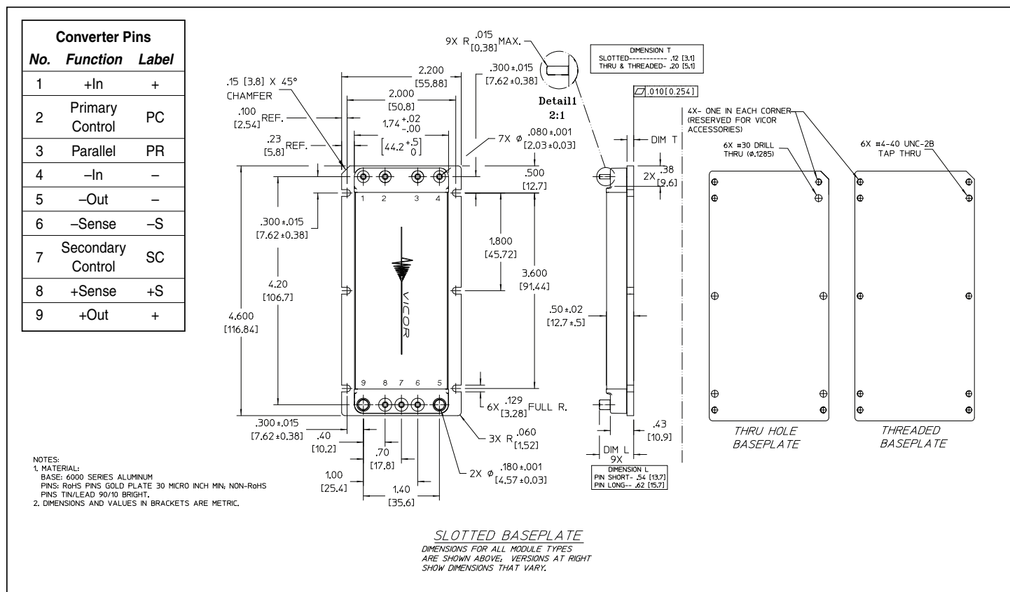
Figure 12 — Module outline
