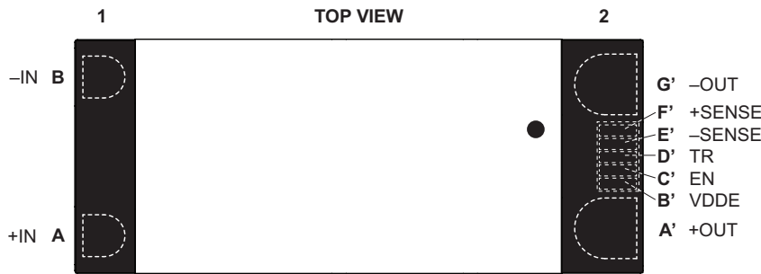
DCM in a VIA package - PCB Mount
