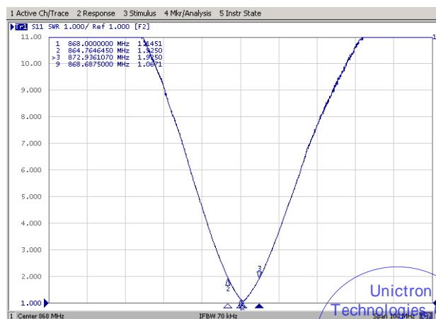
VSWR ( S_{11} )
