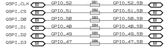
SOLDER BRIDGES
