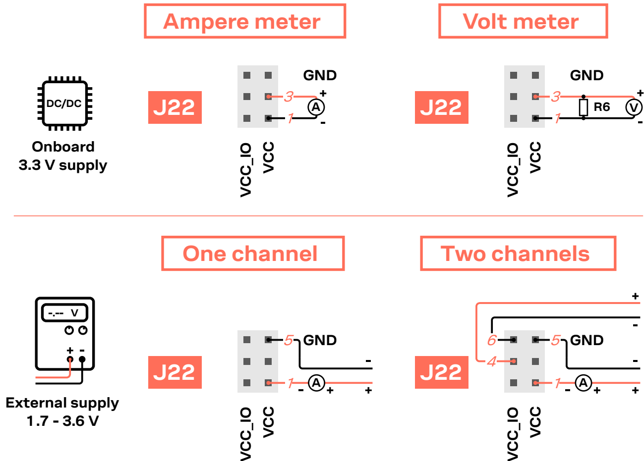
Figure 6: Different options when measuring the NINA module's current consumption
