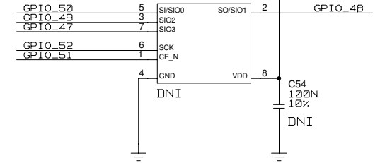
200 MIL PITCH 8-PIN SOP FOOTPRINT FOR EXTERNAL MEMORY
