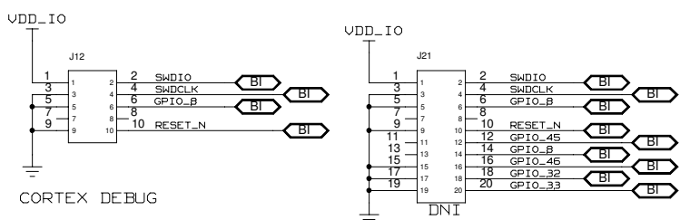
CORTEX DEBUG + ETM DEBUG CONNECTORS
