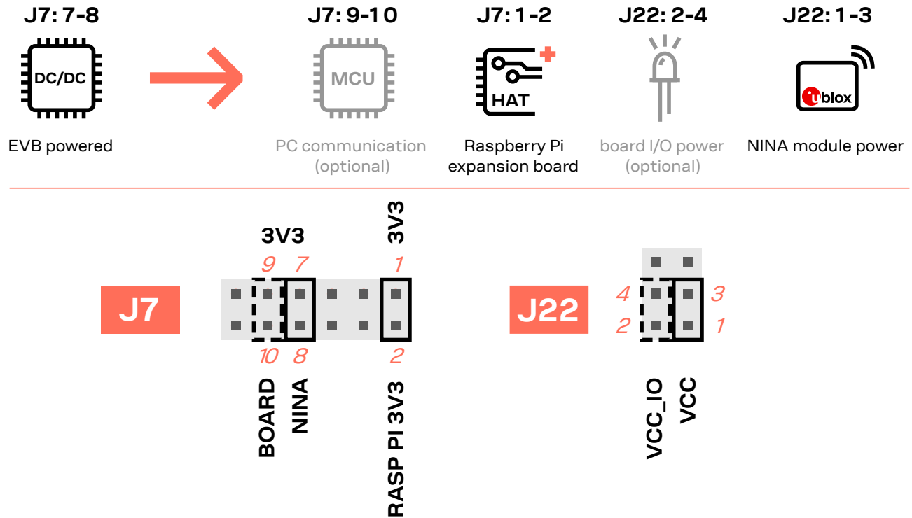
Figure 14: Jumper configuration when connected to a Raspberry Pi HAT, the jumpers shown in dashed lines are optional
