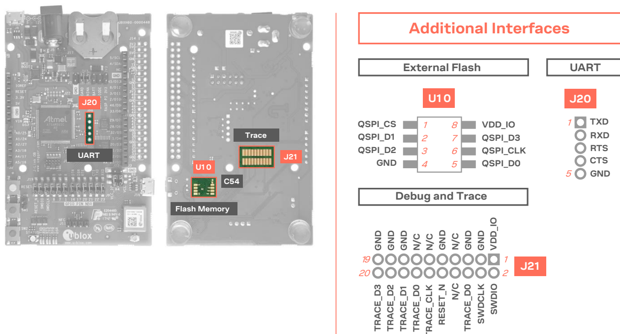
Figure 19: These additional interfaces requires some soldering before use
