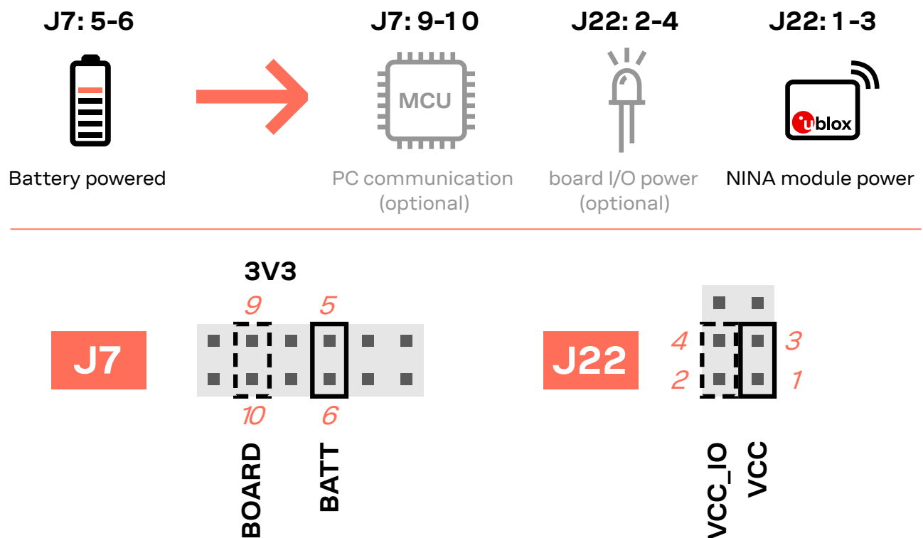
Figure 11: Jumper positions for battery powered operation, the jumpers shown in dashed lines are optional
