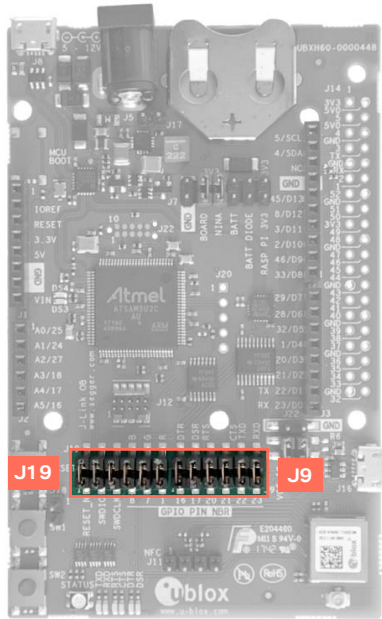
Figure 15: Jumper headers J19 and J9 that are used to isolate specific NINA signals
