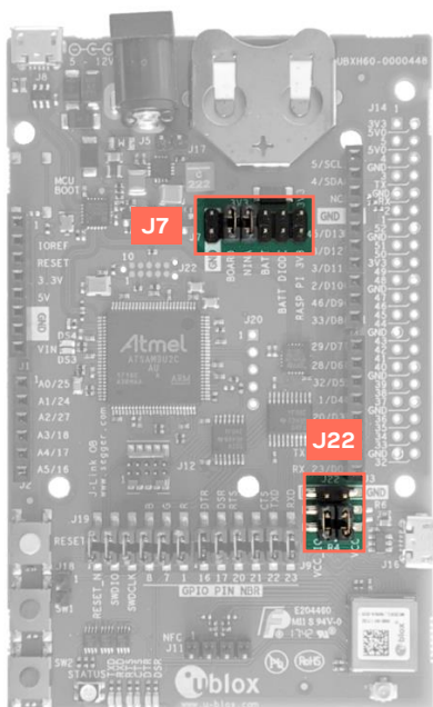
Figure 9: Jumper headers J7 and J22 board location and pinout
