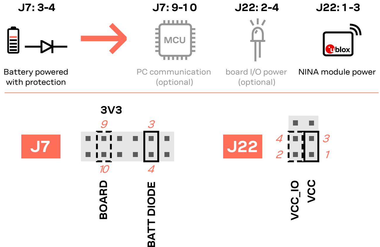
Figure 12: Jumper positions for battery powered operation with a protection diode, the jumpers shown in dashed lines are optional
