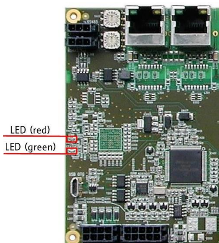
Figure 7.2: LEDs on TMC314 interface brick
