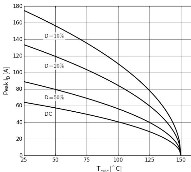
Fig. 8 Maximum Forward Current vs Case Temperature f=10\text{ KHz} (each switch)
