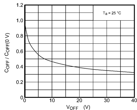
Fig. 12.11 C_{OFF}/C_{OFF(0V)} - V_{OFF}
