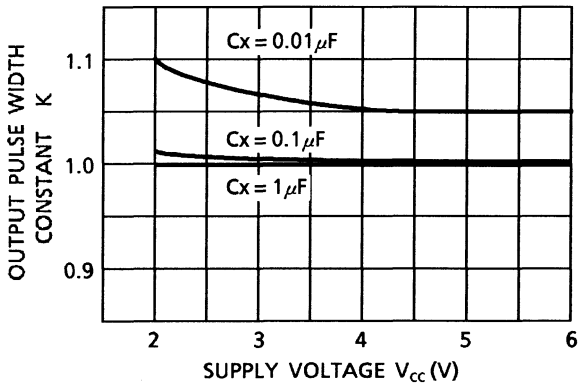
Output Pulse Width Constant K – Supply Voltage (typ.) (EXTERNAL RESISTOR ( R_x ) = 10\text{k}\Omega : t_{\text{WOUT}} = K \cdot C_x \cdot R_x )
