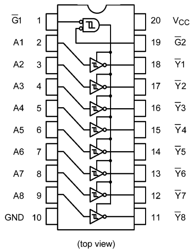
74VHCV540FT
