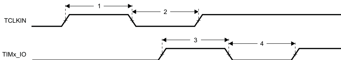
Figure 8-96. Timer Timing
