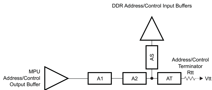
Figure 8-73. ADDR_CTRL Topology for One DDR3 Device
