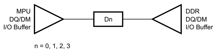
Figure 8-77. DQ/DM Topology
