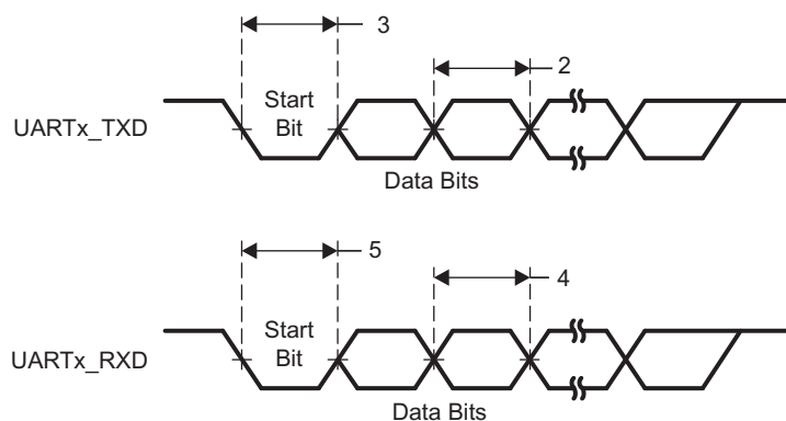
Figure 8-97. UART Timing
