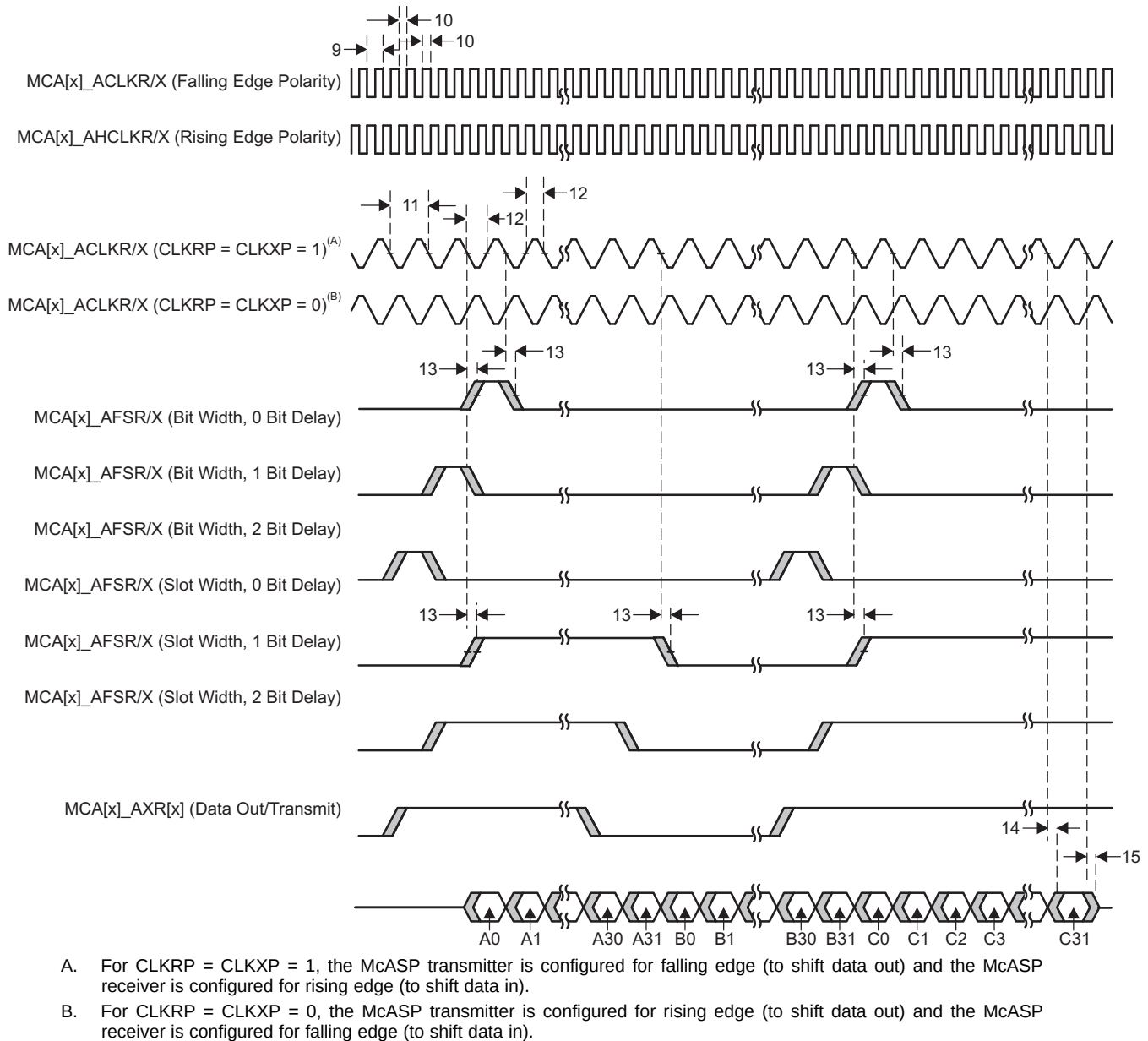
Figure 8-84. McASP Output Timing
