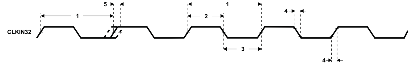
Figure 7-14. CLKIN32 Timing
