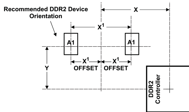
Figure 8-50. AM37x Device and DDR2 Device Placement
