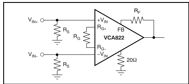
Figure 80. Difference Amplifier
