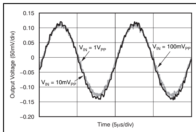
Figure 33. AGC Output Voltage for 100kHz Sinewave at 10mV PP , 100mV PP , and 1V PP
