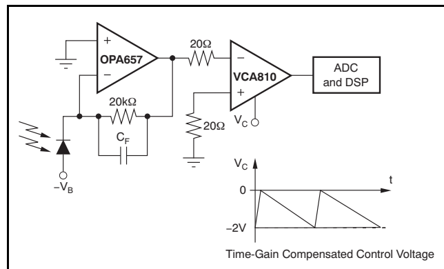
Figure 31. Typical Range-Finding Application
