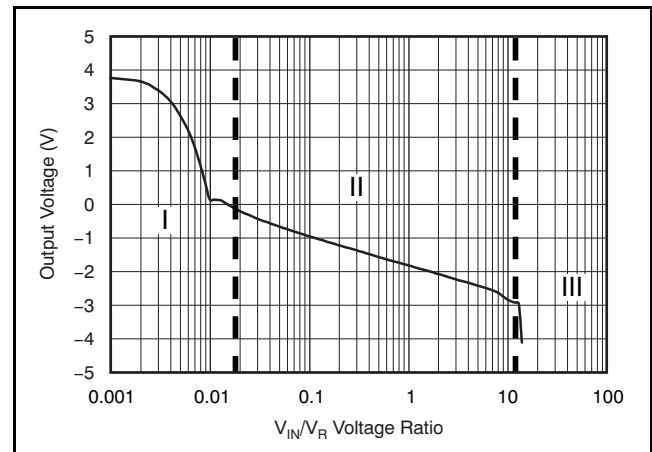
Figure 36. Test Result for LOG Amp for V_R = -100\text{mV}
