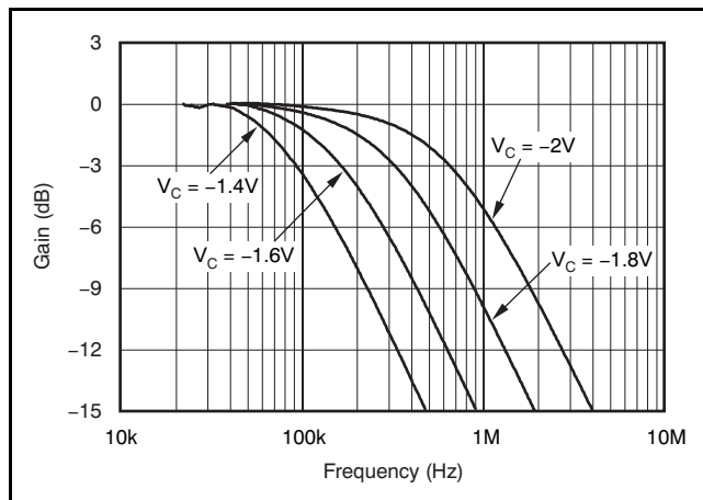
Figure 40. Voltage-Controlled Low-Pass Filter Frequency Response
