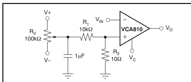
Figure 46. Optional Offset Adjustment
