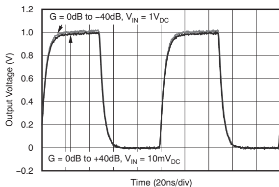
GAIN CONTROL PULSE RESPONSE
