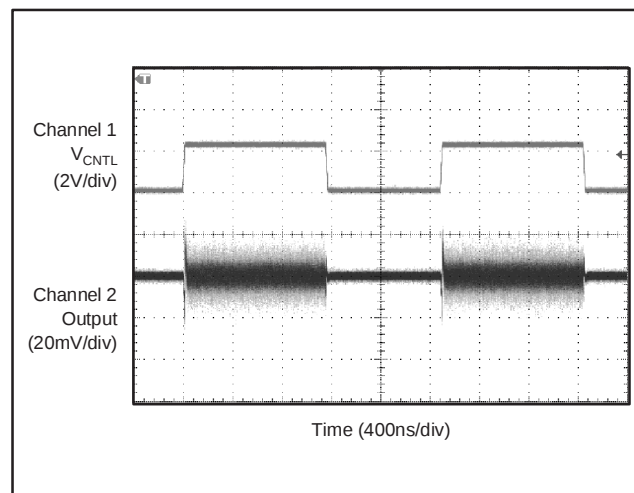
Figure 37. Response to Step Change of V_{CTL}
