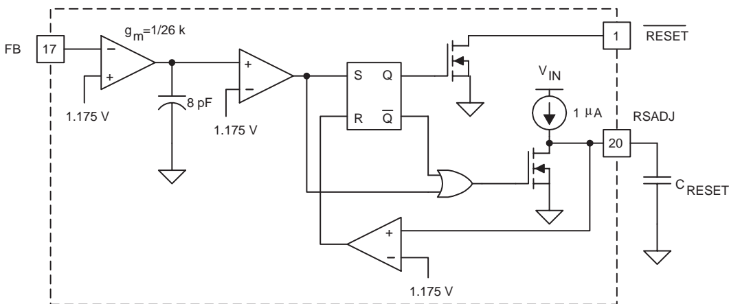
Figure 17. Reset Circuitry
