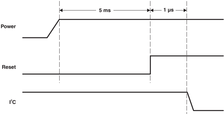
Figure 7. Reset Timing
