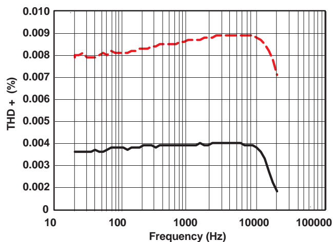
Figure 13. Total Harmonic Distortion vs Frequency (V + = 5 V)
