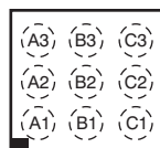
TPS7510x YFF 9-Ball WCSP (Top View)
