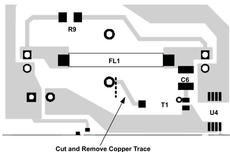
Figure 1. TPS65560EVM-165 Top Layer
